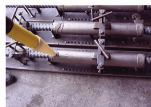
Assembling test specimens in the temperature controlled curing room
